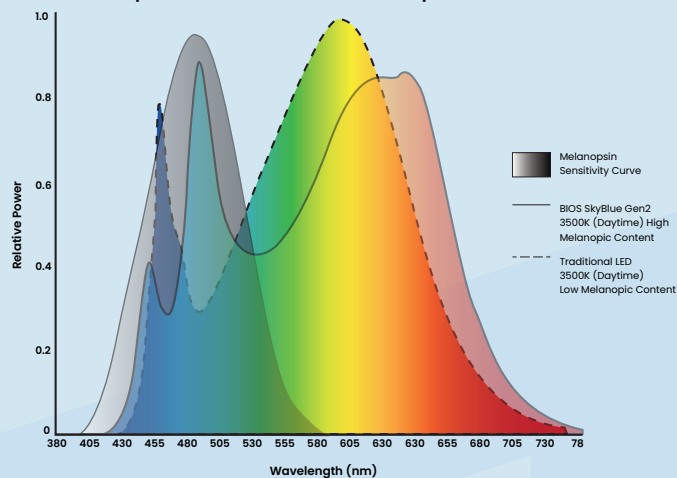
BIOS Static BlueSky™ Gen 2 vs Traditional White Light Spectral Power Distribution Comparison
