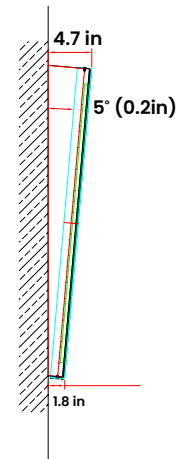
Tilt Mount Bracket Accessory (For Rectangular Mirror Only)
