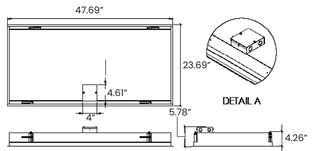
SCR (W/OC FRAME) RECESSED GRID SCR (W/OC FRAME) RECESSED FLANGE
